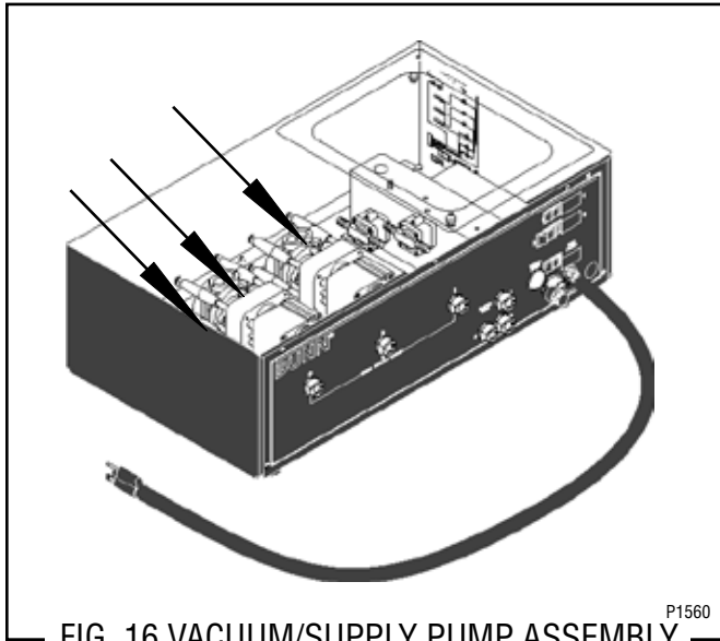
FIG. 16 VACUUM/SUPPLY PUMP ASSEMBLY P1560
