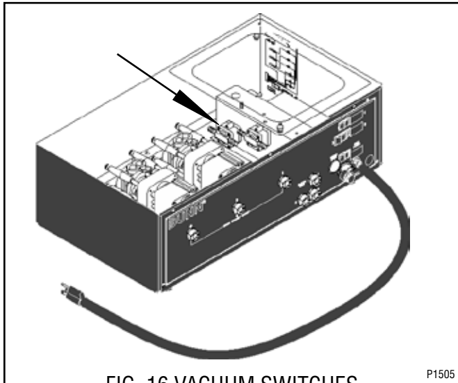
FIG. 16 VACUUM SWITCHES
