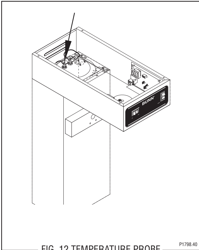
FIG. 12 TEMPERATURE PROBE
