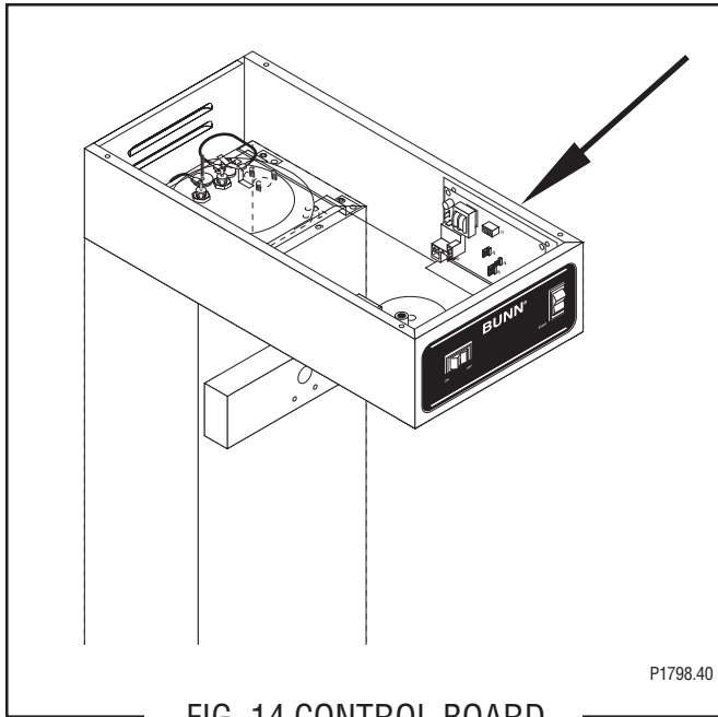
FIG. 14 CONTROL BOARD
