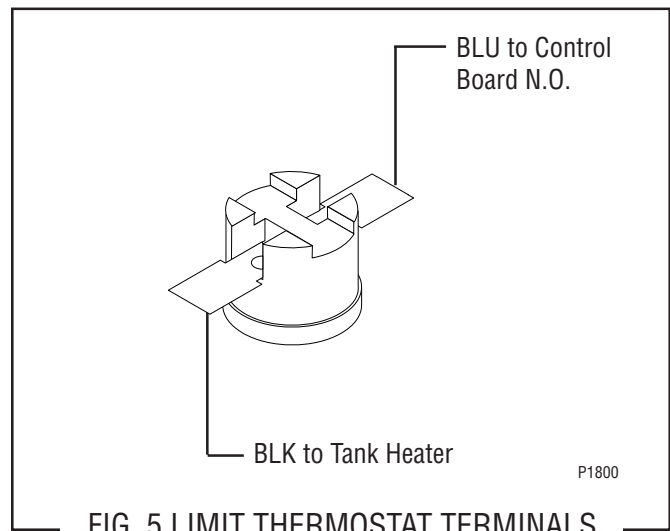
FIG. 5 LIMIT THERMOSTAT TERMINALS
